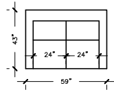
LOVE SEAT W: 59" D: 43" H: 38" ARM H: 27" SEAT D: 21"
