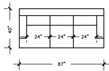
SOFA W: 87" D: 40" H: 34" ARM H: 25" SEAT D: 23"
