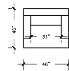
CHAIR & HALF W: 46" D: 40" H: 34" ARM H: 25" SEAT D: 23"
